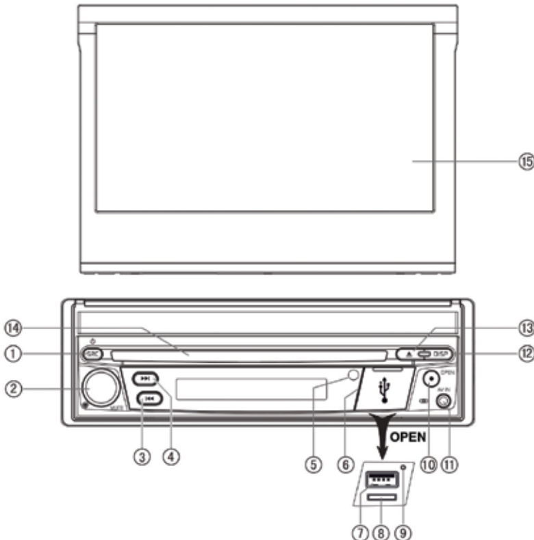
Figure 1: MAC 410 Controls and Indicators
