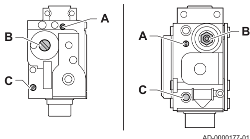
Abb.43 Gasarmaturen
