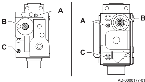
Abb.44 Gasarmaturen
