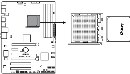
M5A97 R2.0 CPU socket AM3+
