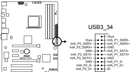
M5A97 R2.0 USB3.0 Front panel connector
