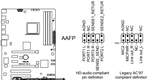
M5A97 R2.0 Front panel audio connector
