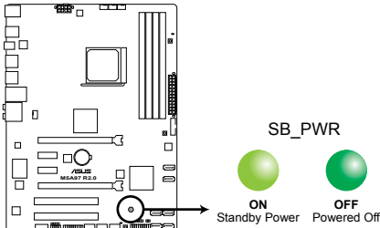
M5A97 R2.0 Onboard LED
