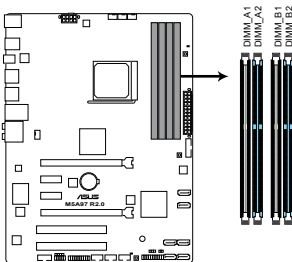
M5A97 R2.0 240-pin DDR3 DIMM sockets
