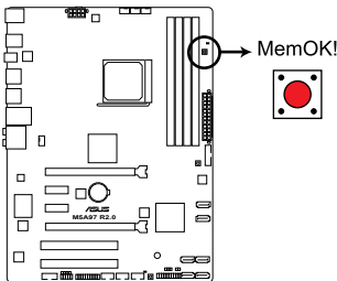
M5A97 R2.0 MemOK! switch
