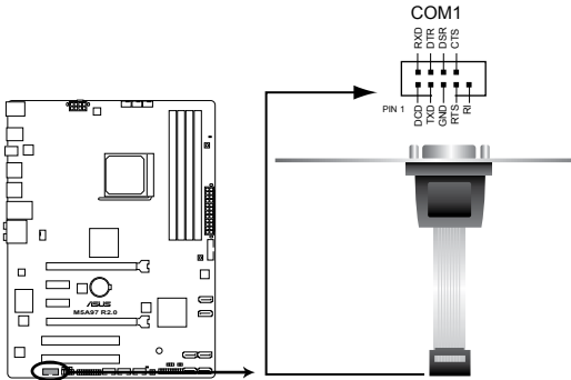
M5A97 R2.0 Serial port (COM1) connector
