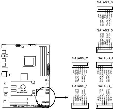
M5A97 R2.0 SATA 6.0Gb/s connectors
