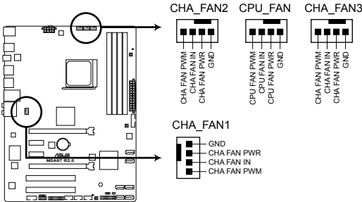
M5A97 R2.0 Fan connectors
