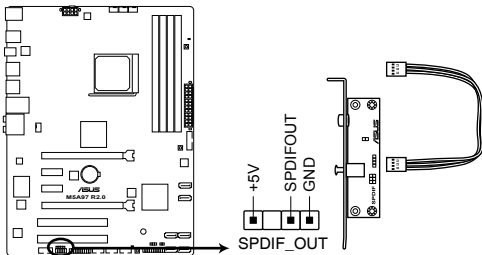
M5A97 R2.0 Digital audio connector
