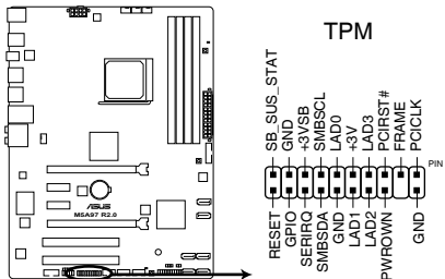
M5A97 R2.0 TPM Connector
